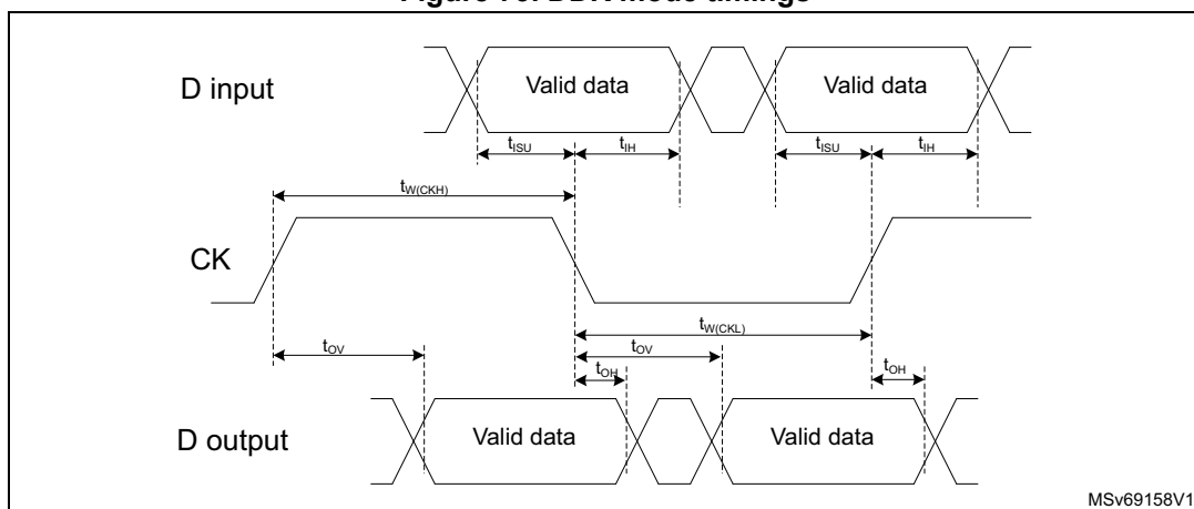
Figure 73. DDR mode timings
