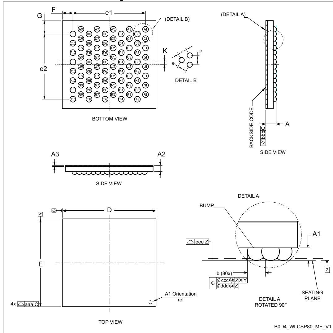
Figure 83. WLCSP80 - Outline
