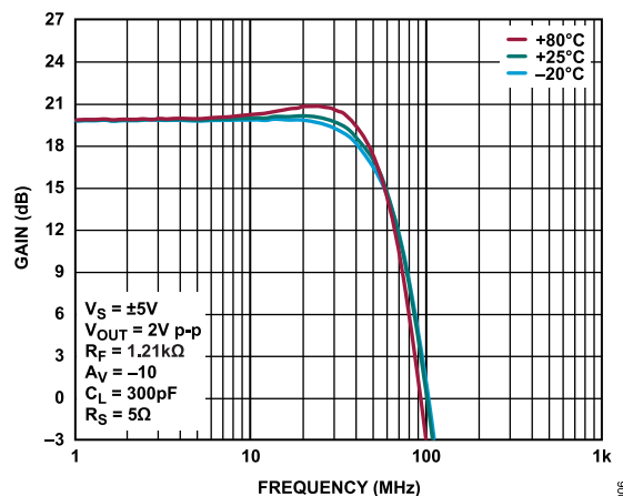
Figure 6. Small Signal Frequency Response vs. Case Temperature, A_V = -10 , V_S = \pm 5\text{ V} , V_{\text{OUT}} = 2\text{ V p-p} , R_F = 1.21\text{ k}\Omega , C_L = 300\text{ pF} , R_S = 5\text{ }\Omega
