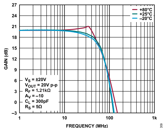
Figure 9. Large Signal Frequency Response vs. Case Temperature, A_V = -10 , V_S = \pm 20\text{ V} , V_{\text{OUT}} = 20\text{ V p-p} , R_F = 1.21\text{ k}\Omega , C_L = 300\text{ pF} , R_S = 5\text{ }\Omega
