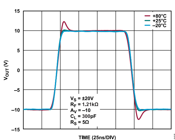
Figure 27. Large Signal Pulse Response vs. Case Temperature, A_V = -10 , V_S = \pm 20 V, V_{OUT} = 20 V p-p, R_F = 1.21 k \Omega , C_L = 300 pF, R_S = 5 \Omega
