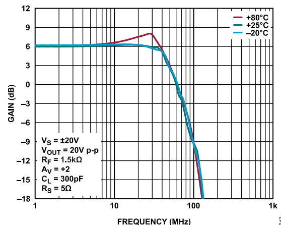
Figure 13. Large Signal Frequency Response vs. Case Temperature, A_V = +2 , V_S = \pm 20 V, V_{OUT} = 20 V p-p, R_F = 1.5 k \Omega , C_L = 300 pF, R_S = 5 \Omega
