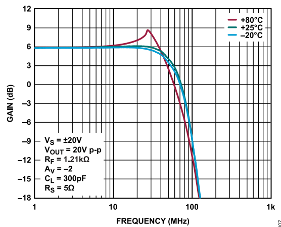
Figure 7. Large Signal Frequency Response vs. Case Temperature, A_V = -2 , V_S = \pm 20\text{ V} , V_{\text{OUT}} = 20\text{ V p-p} , R_F = 1.21\text{ k}\Omega , C_L = 300\text{ pF} , R_S = 5\text{ }\Omega
