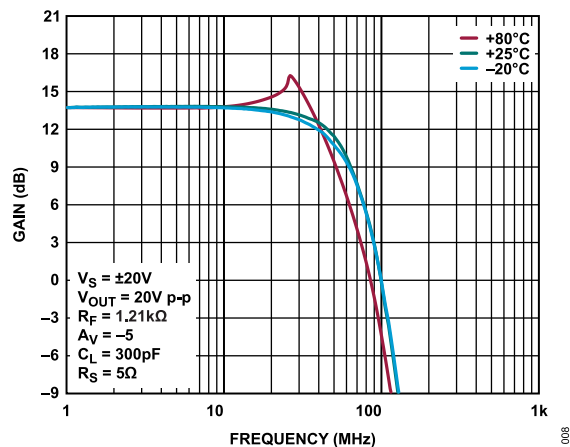
Figure 8. Large Signal Frequency Response vs. Case Temperature, A_V = -5 , V_S = \pm 20\text{ V} , V_{\text{OUT}} = 20\text{ V p-p} , R_F = 1.21\text{ k}\Omega , C_L = 300\text{ pF} , R_S = 5\text{ }\Omega
