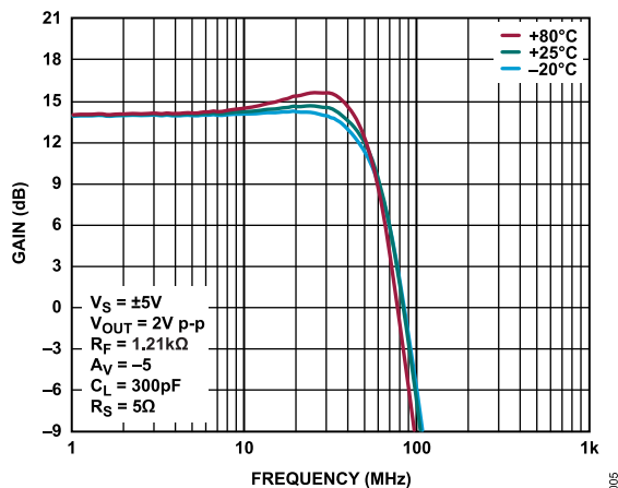
Figure 5. Small Signal Frequency Response vs. Case Temperature, A_V = -5 , V_S = \pm 5\text{ V} , V_{\text{OUT}} = 2\text{ V p-p} , R_F = 1.21\text{ k}\Omega , C_L = 300\text{ pF} , R_S = 5\text{ }\Omega
