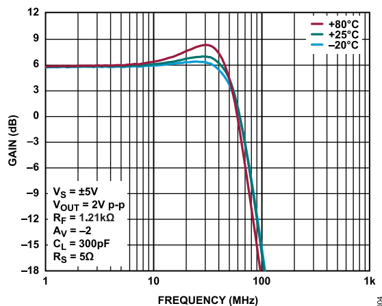
Figure 4. Small Signal Frequency Response vs. Case Temperature, A_V = -2 , V_S = \pm 5\text{ V} , V_{\text{OUT}} = 2\text{ V p-p} , R_F = 1.21\text{ k}\Omega , C_L = 300\text{ pF} , R_S = 5\text{ }\Omega
