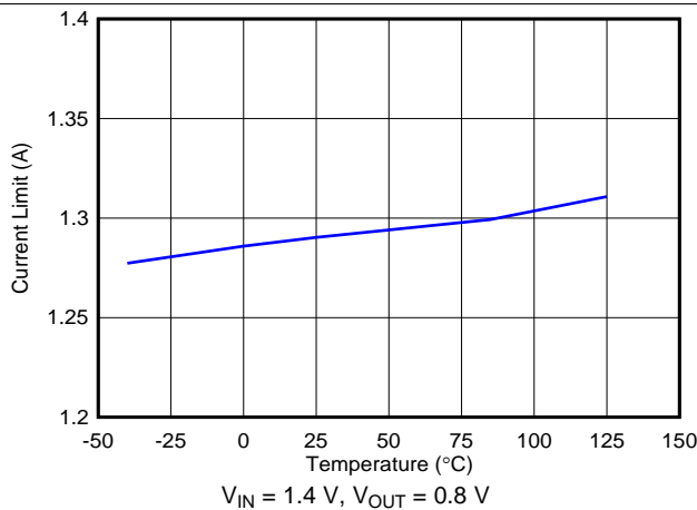
图 13. Current Limit vs Temperature
