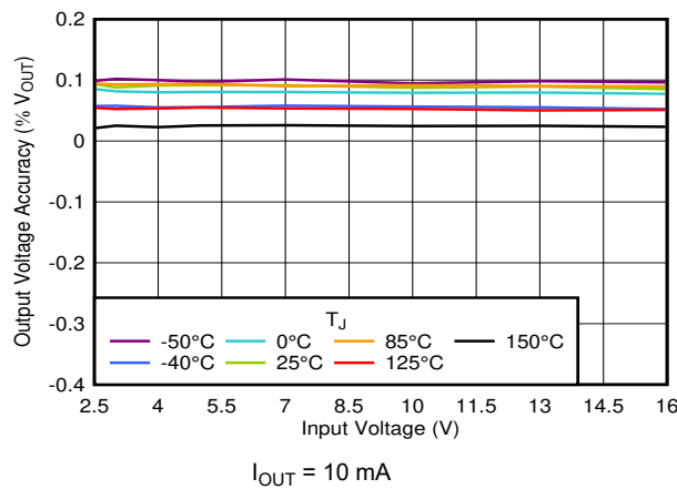
图 6-3. V_{OUT} Accuracy vs V_{IN}
