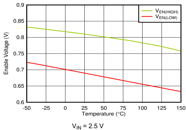
图 6-23. V_{EN} Thresholds vs Temperature
