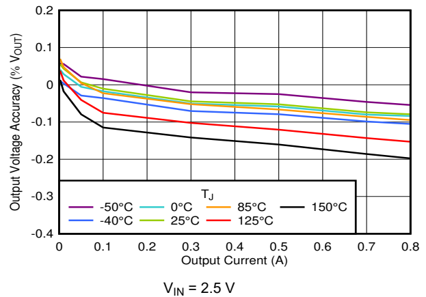
图 6-2. V_{OUT} Accuracy vs I_{OUT}
