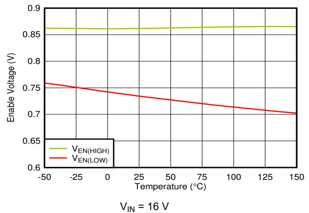
图 6-24. V_{EN} Thresholds vs Temperature
