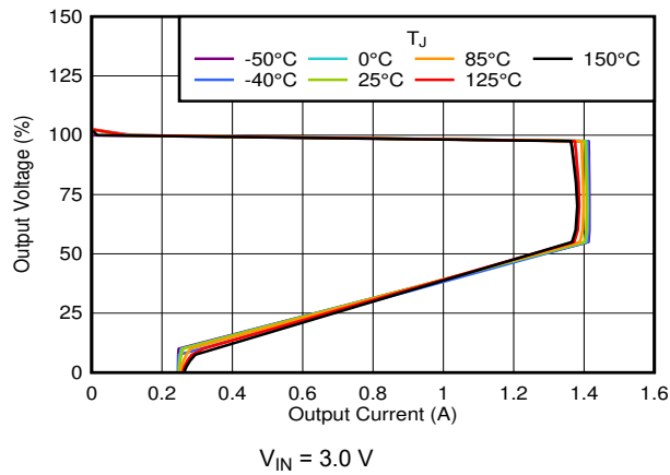
图 6-19. Foldback Current Limit vs I_{OUT} and Temperature
