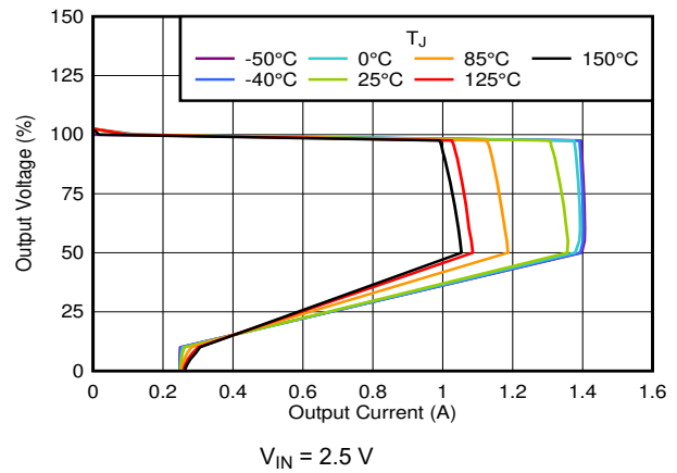
图 6-20. Foldback Current Limit vs I_{OUT} and Temperature
