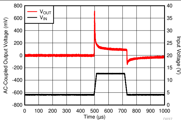
图 6-13. V_{IN} Transient in Dropout From 4 V to 13 V
