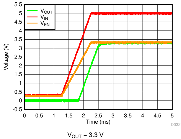
图 6-21. Startup With Separate V_{EN} and V_{IN}
