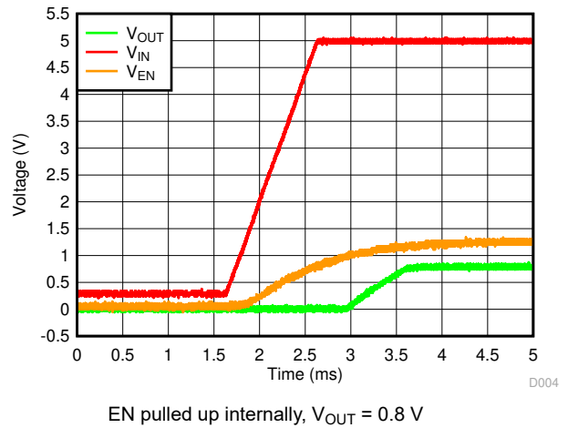
图 6-22. Startup With V_{EN} Floating
