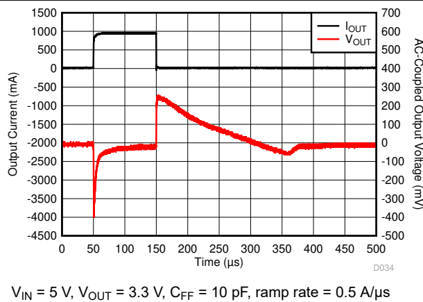
图 6-11. I_{OUT} Transient From 1 mA to 1 A
