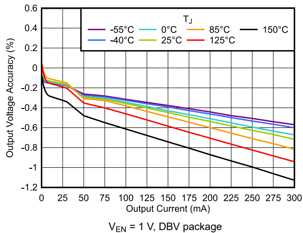
图 5-15. Output Voltage Accuracy vs I_{OUT}
