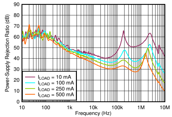
图 5-32. PSRR vs Frequency and I_{LOAD}
