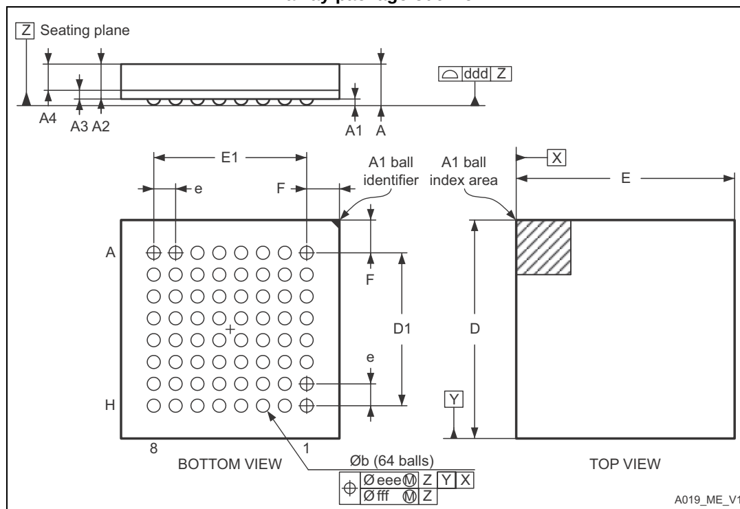
Figure 41. UFBGA64 – 64-ball, 5 x 5 mm, 0.5 mm pitch ultra profile fine pitch ball grid array package outline
